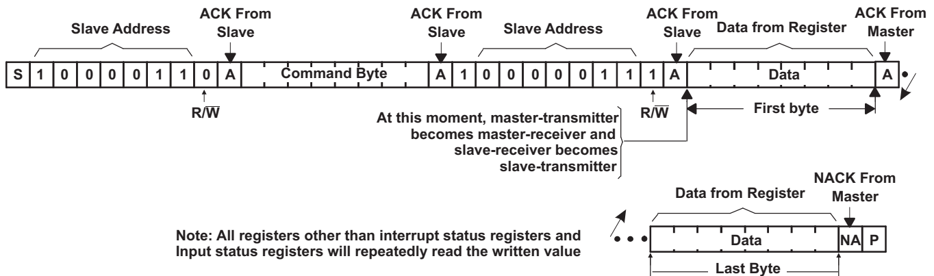
Figure 12. Read From Register
