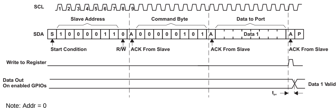
Figure 10. Write To Output State Register
