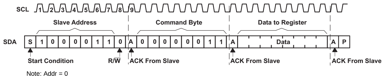
Figure 11. Write To I/O Direction Register
