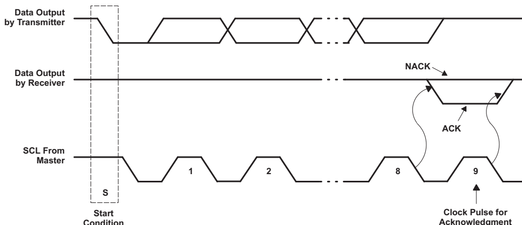
Figure 9. Acknowledgment on I²C Bus
