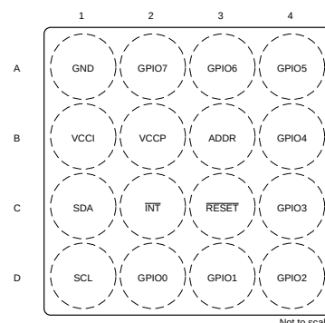
ZSZ Package (Top Through View)
