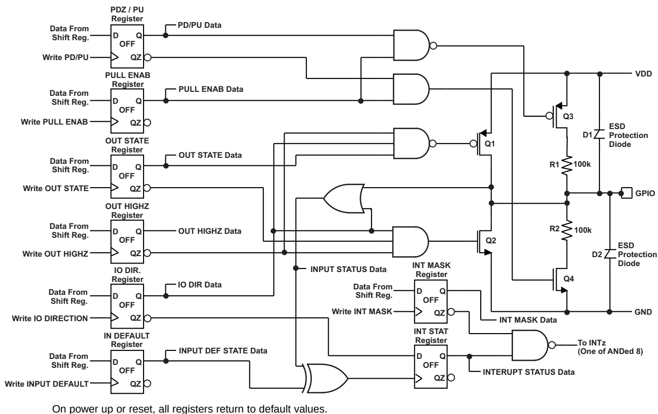
Figure 5. Simplified Logic Diagram (Positive Logic)
